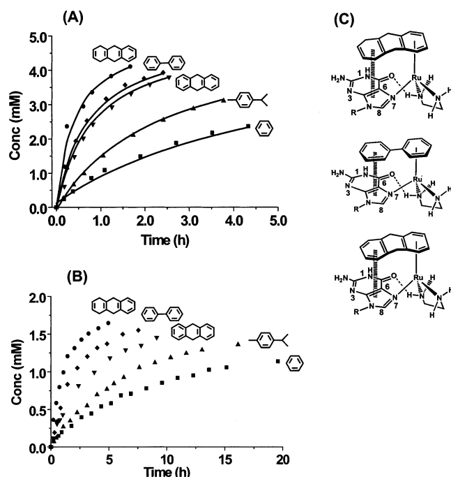
Figure 6. Plots showing the variation of the concentration of (\eta^6\text{-arene})\text{-Ru-N7cGMP} products with time during the reaction of (A) [(\eta^6\text{-arene})\text{Ru}(\text{en})(\text{H}_2\text{O})]^{2+} (5 mM), (B) [(\eta^6\text{-arene})\text{Ru}(\text{en})\text{Cl}]^+ (2 mM) with cGMP (1:1, pH 7.0), 100 mM \text{NaClO}_4 , 298 K, based on the integration of G H8 ^1\text{H} NMR peaks. The curves in (A) are computer-fits to second-order kinetics giving the rate constants listed in Table 6. These reactions were all followed for periods of between 24 h and 4 days (see Figures S8 and S9). The reactions of the chloro complexes in (B) were followed for up to 1 week, and the half-lives for the formation of Ru–N7 adducts are shown in Table 6. No attempt was made to fit these data and determine the rate constants. (C) Possible \pi\text{-}\pi stacking between arene and purine in cGMP adducts with Ru(THA), Ru(Bip), and Ru(DHA).
