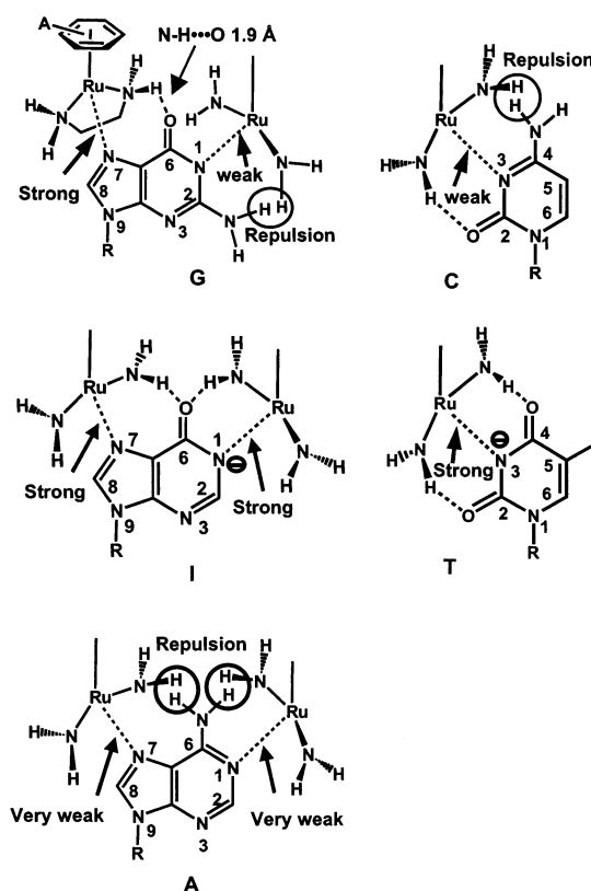
Figure 5. Regio- and stereo-specificities: H-bonds and nonbonding repulsions for the interaction of \{(\eta^6\text{-arene})\text{Ru}(\text{en})\}^{2+} with nucleobases, as detected in nucleoside and nucleotide reactions. For clarity, the arene and the \text{CH}_2\text{CH}_2 of the en ring have been omitted, except for the G adduct. For the purine adducts, the diagrams indicate in a general way the reactions with N7 and N1 and are not intended to apply specifically to the dinuclear adducts.
